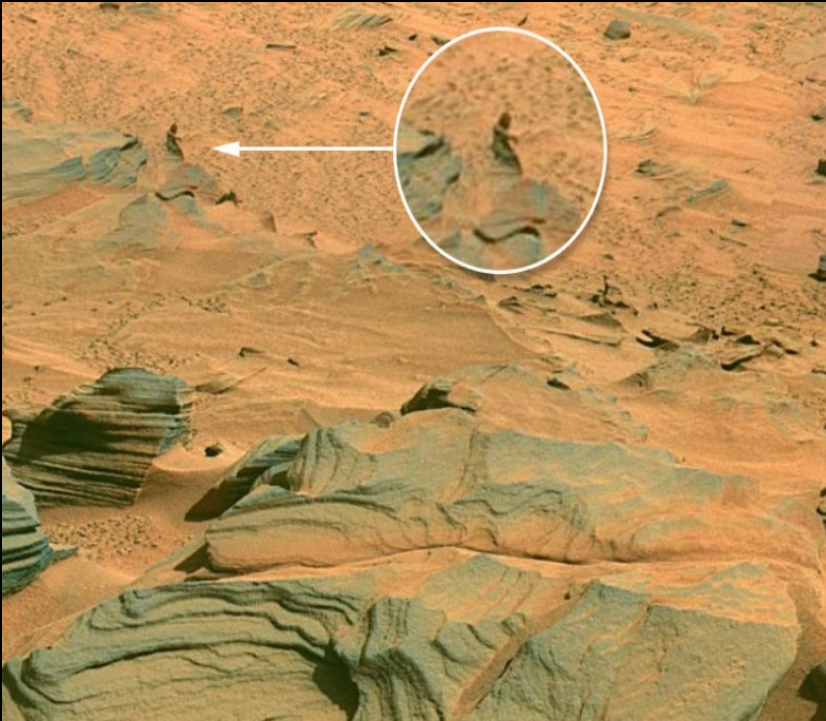
Mars, Spirit, 2008
